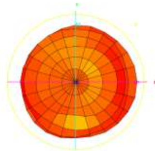
Total_3D_Side View_1.88GHz
