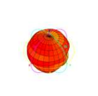
Total_3D_Side View_1.71GHz
